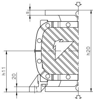
Non-drive end view / Vista lato opposto comando
