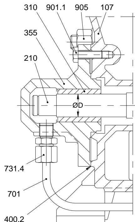
Fig. 2 - Sectional drawing sleeve bearing housing
